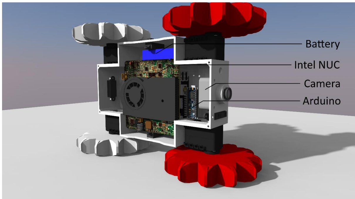
Figure 22 - Internal Components
