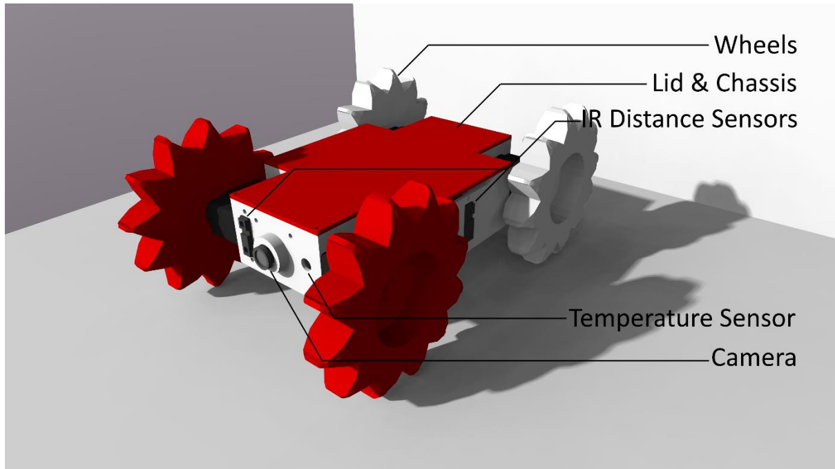
Figure 21 - External Components
